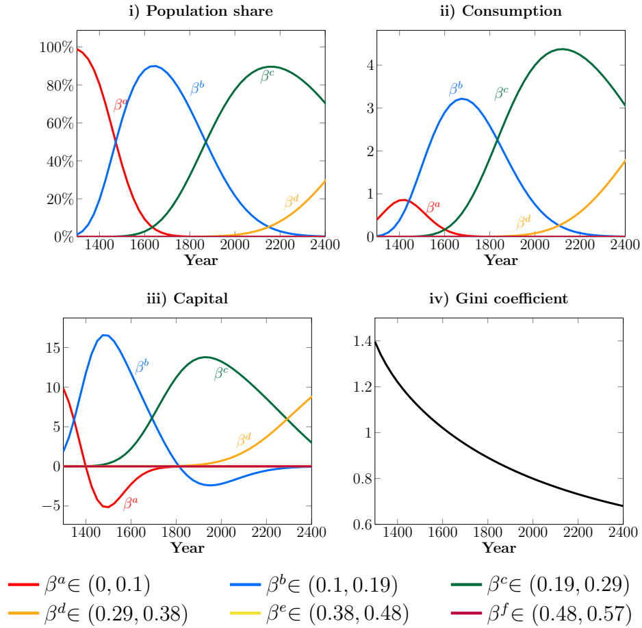
Figure 4: Characteristics of groups and inequality over 1300–2100
