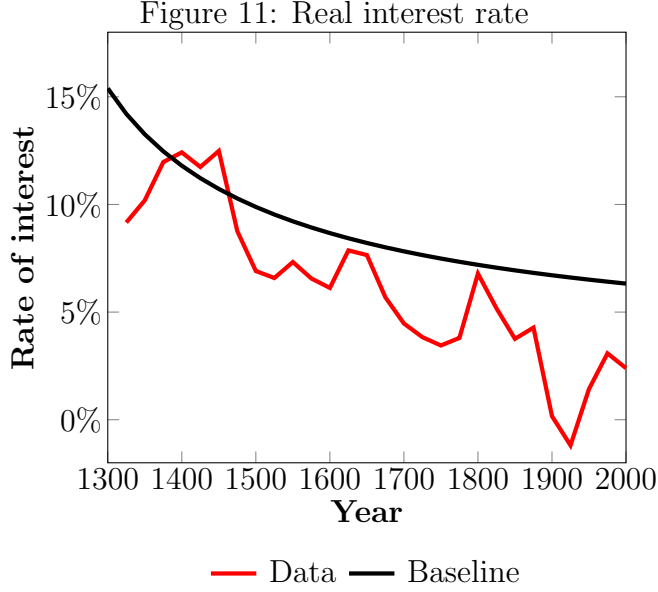
Data is the Schmelzing (2020) global real interest rate. Baseline is the model in section 3.
